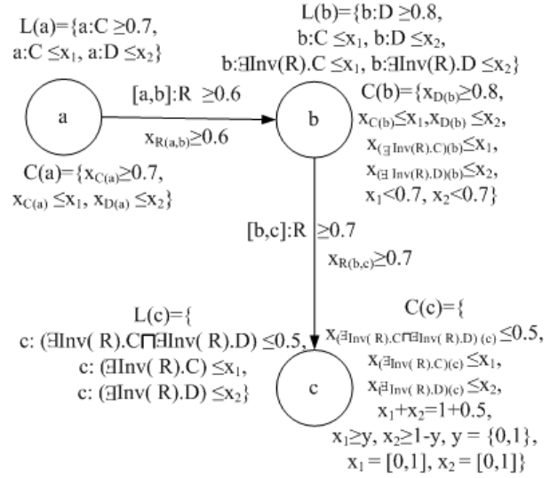
Figure 2: The extended fuzzy tableau of example 3.
